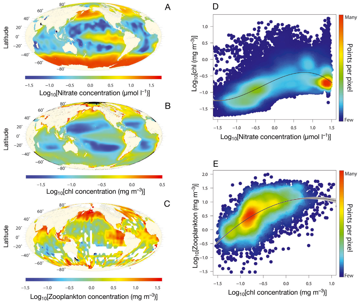
Fig. 6. Global climatology of phytoplankton, zooplankton, and nutrient concentrations. Averaged (A) nitrate, (B) chlorophyll, and (C) zooplankton concentration per 1^\circ \times 1^\circ cell depicted as colors. White represents areas with no data. (D) Chlorophyll and (E) zooplankton concentration as a function of nitrate, and (E) zooplankton as a function of chlorophyll. All variables are \text{log}_{10} -transformed average concentrations per 1^\circ \times 1^\circ cell. Colors depict the number of measurements per pixel. Relationship in (D) was best approximated by a polynomial function, and relationship in (E) was best approximated by a quadratic function. Shading represents the 95% confidence limits around the fitted curve
